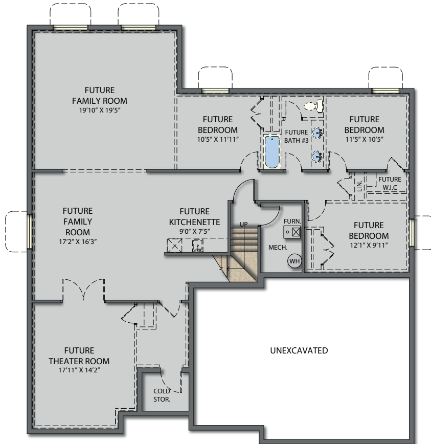
BASEMENT FLOOR
