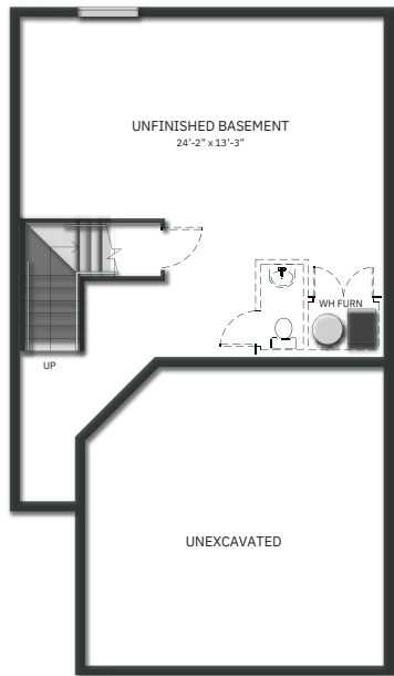
Basement Floor
